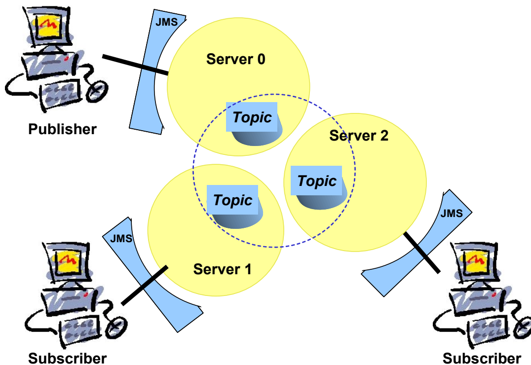
Figure 20 - Cluster sample configuration
